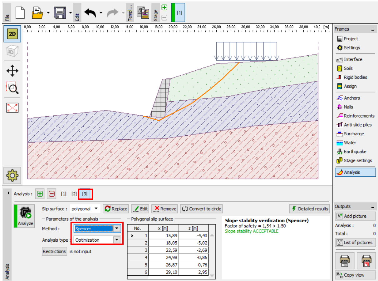
Frame "Analysis" – Spencer – optimization of a polygonal slip surface
