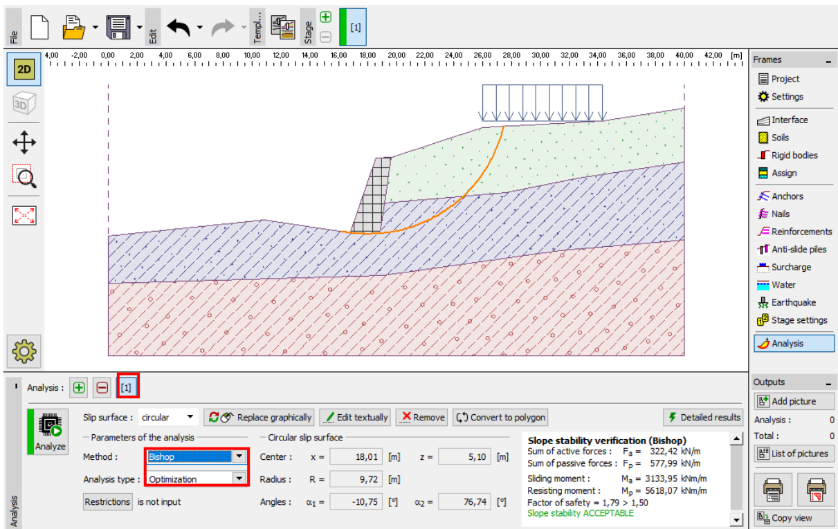
Frame “Analysis” – Bishop – optimization of circular slip surface
