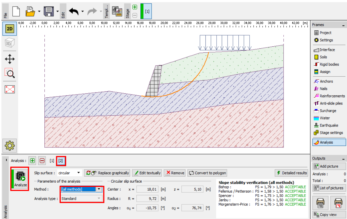
Frame “Analysis” – All methods – standard type of analysis
