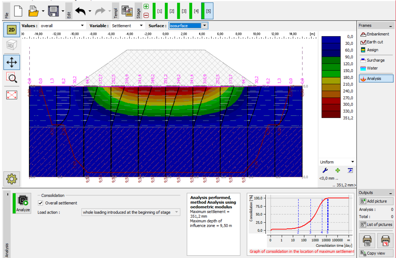
Frame "Analysis – Construction Stage 5"
