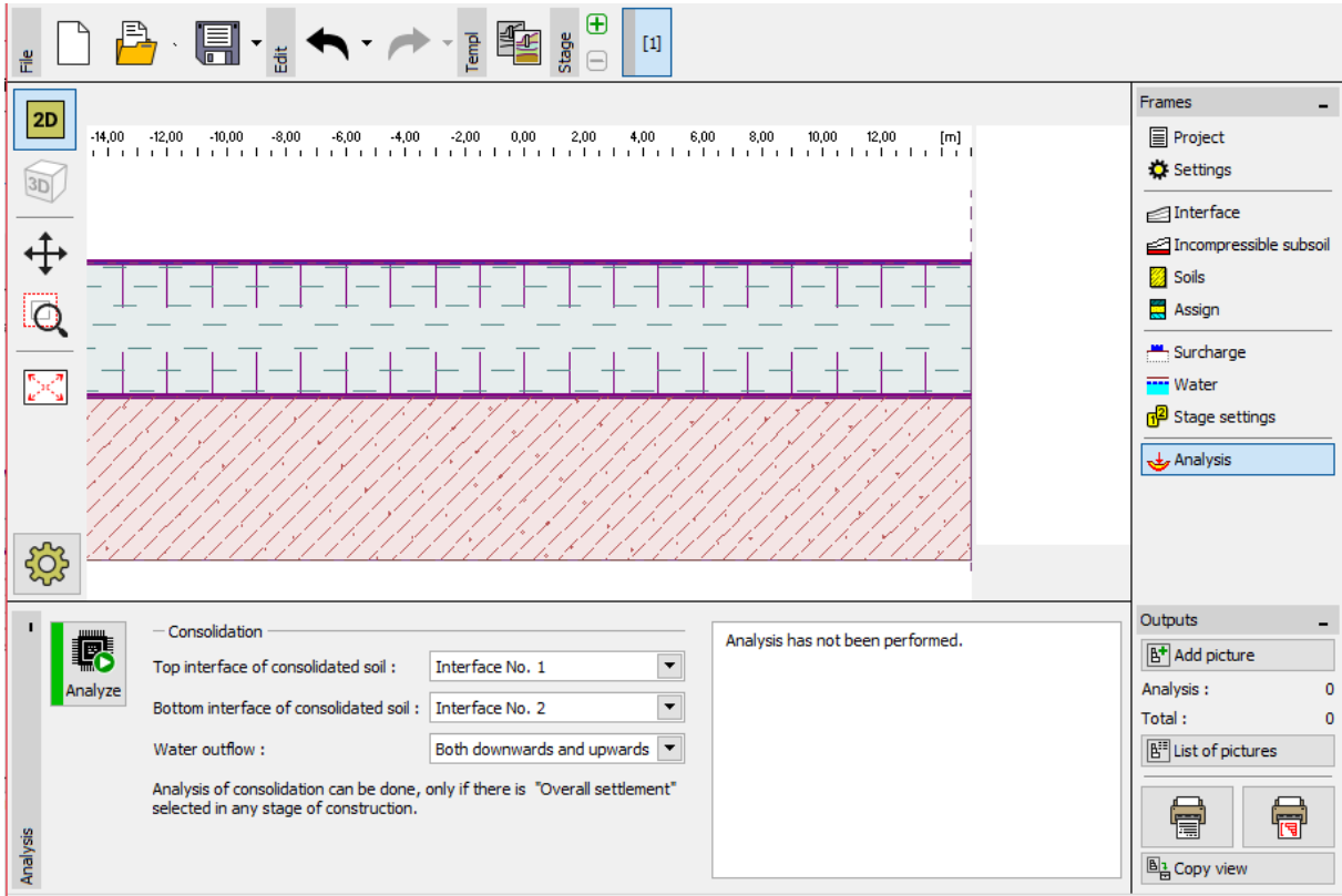
"Analysis" settings – Construction stage 1
