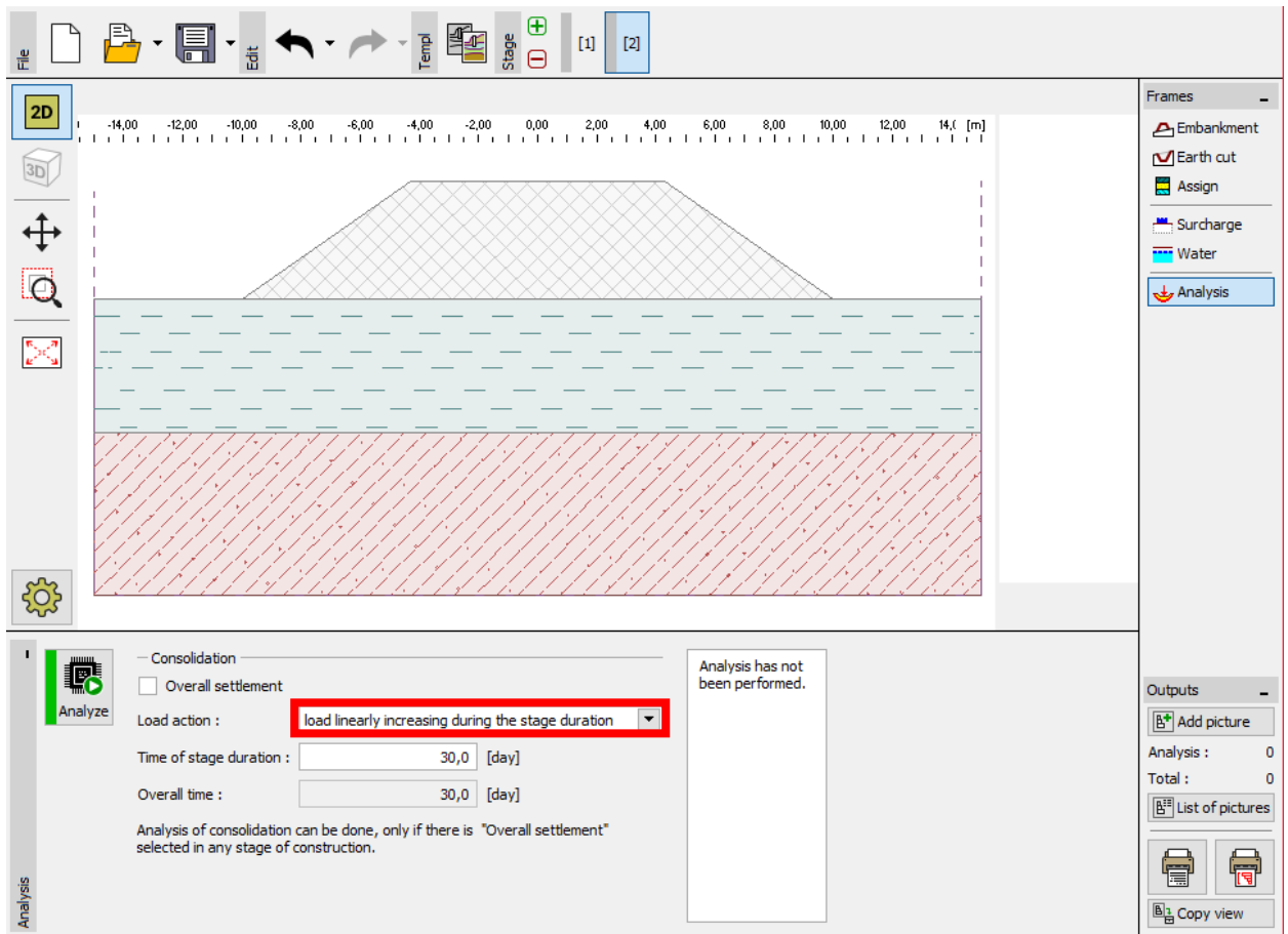
Frame "Analysis – Construction Stage 2"
