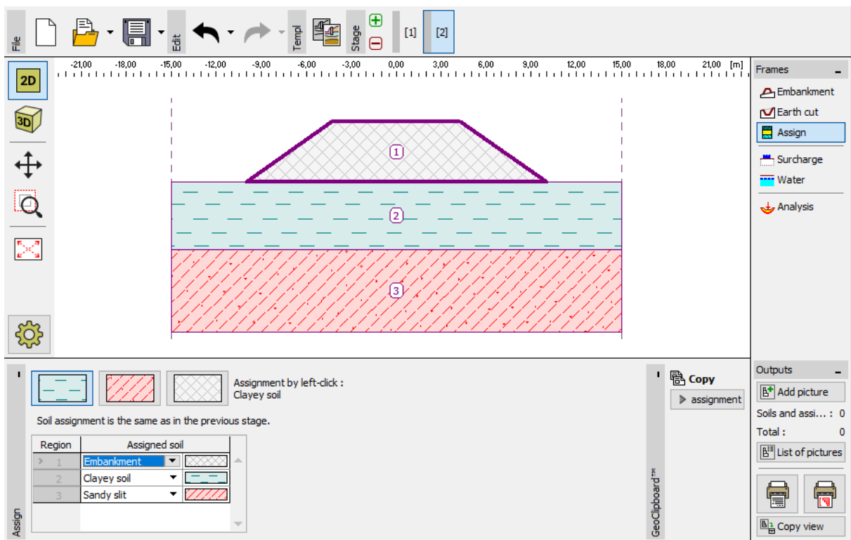
"Stage 2 – Embankment + Assignment"
