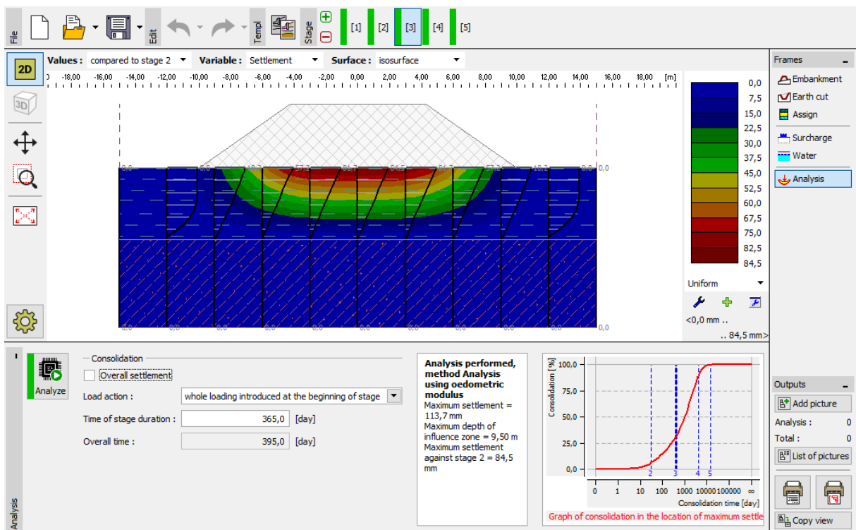
Frame "Analysis" – Settlement (differences compared to previous stages)
