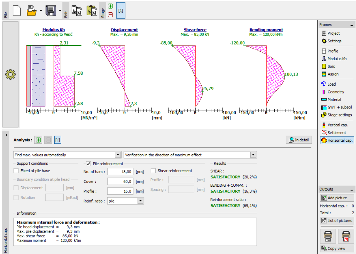
Frame “Horizontal bearing capacity” - Course of modulus of horizontal reaction of subsoil k_h according to Vesic, deformation and internal forces
