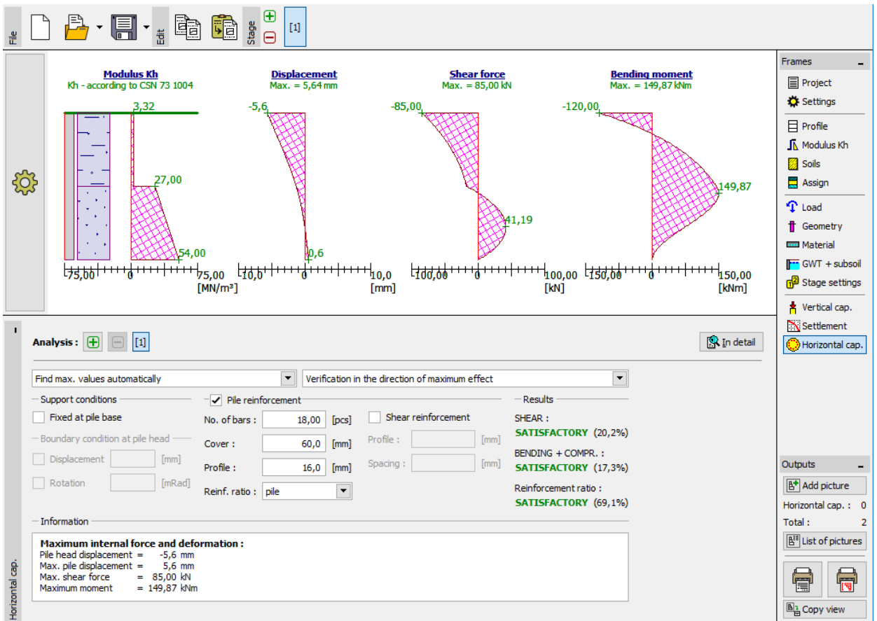
Frame “Horizontal bearing capacity” - Course of modulus of subsoil reaction k_h according to CSN 73 1004, deformation and internal forces
