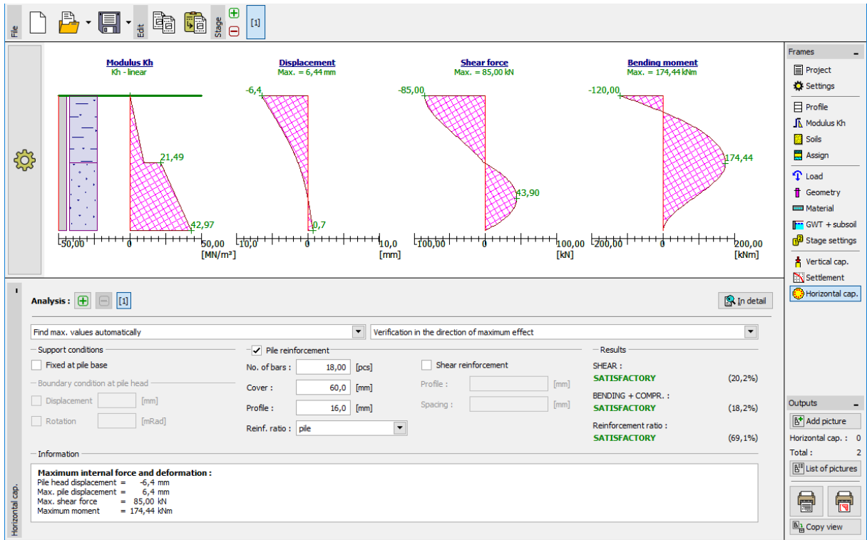
Frame "Horizontal bearing capacity" - Linear course of the modulus of horizontal reaction of subsoil k_h , deformation and internal forces
