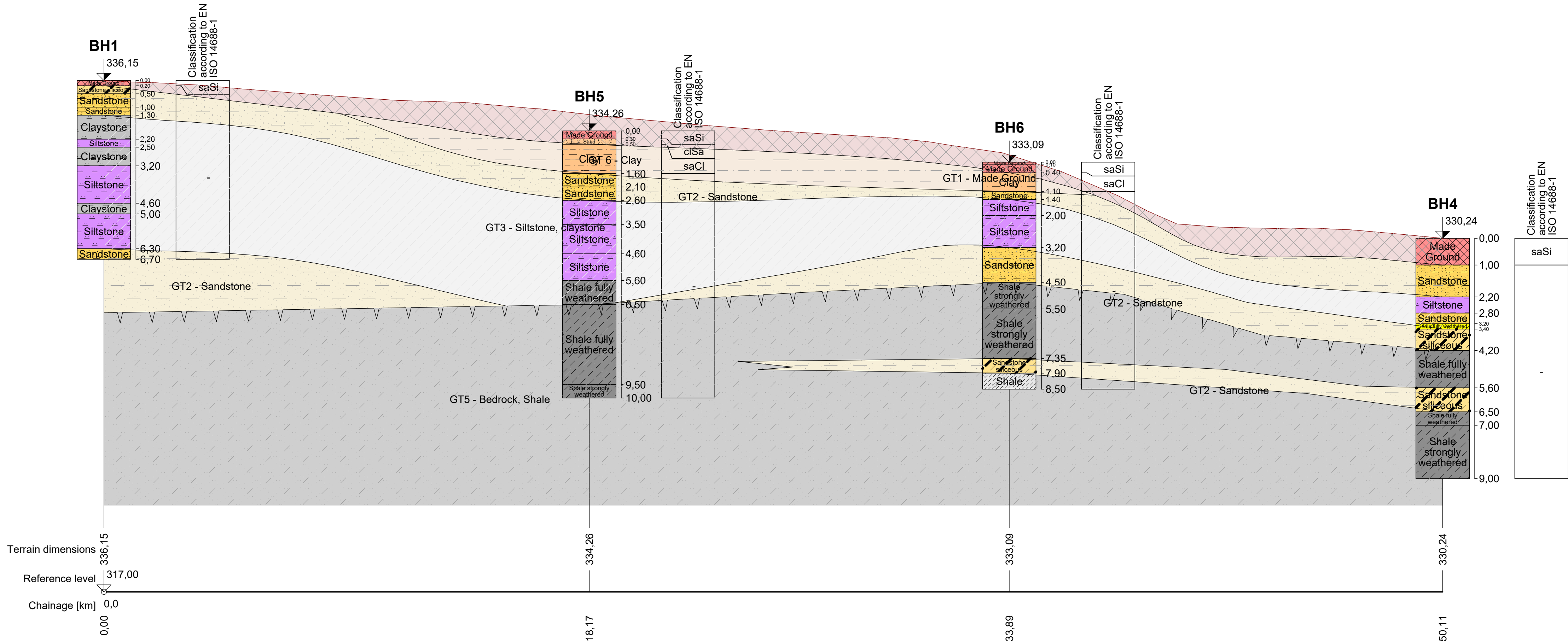
GEOLOGICAL SECTION S 1:100/100
