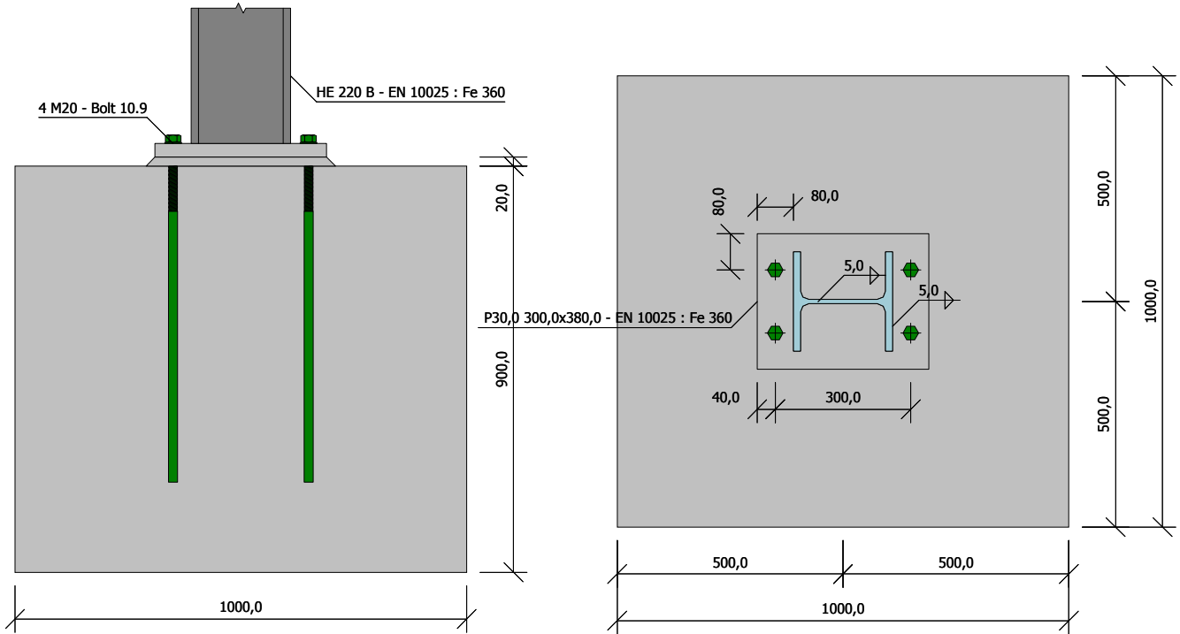
column base: Stiff end plate
