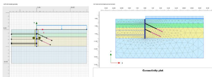
PLAXIS geometry at the adopted support section.
